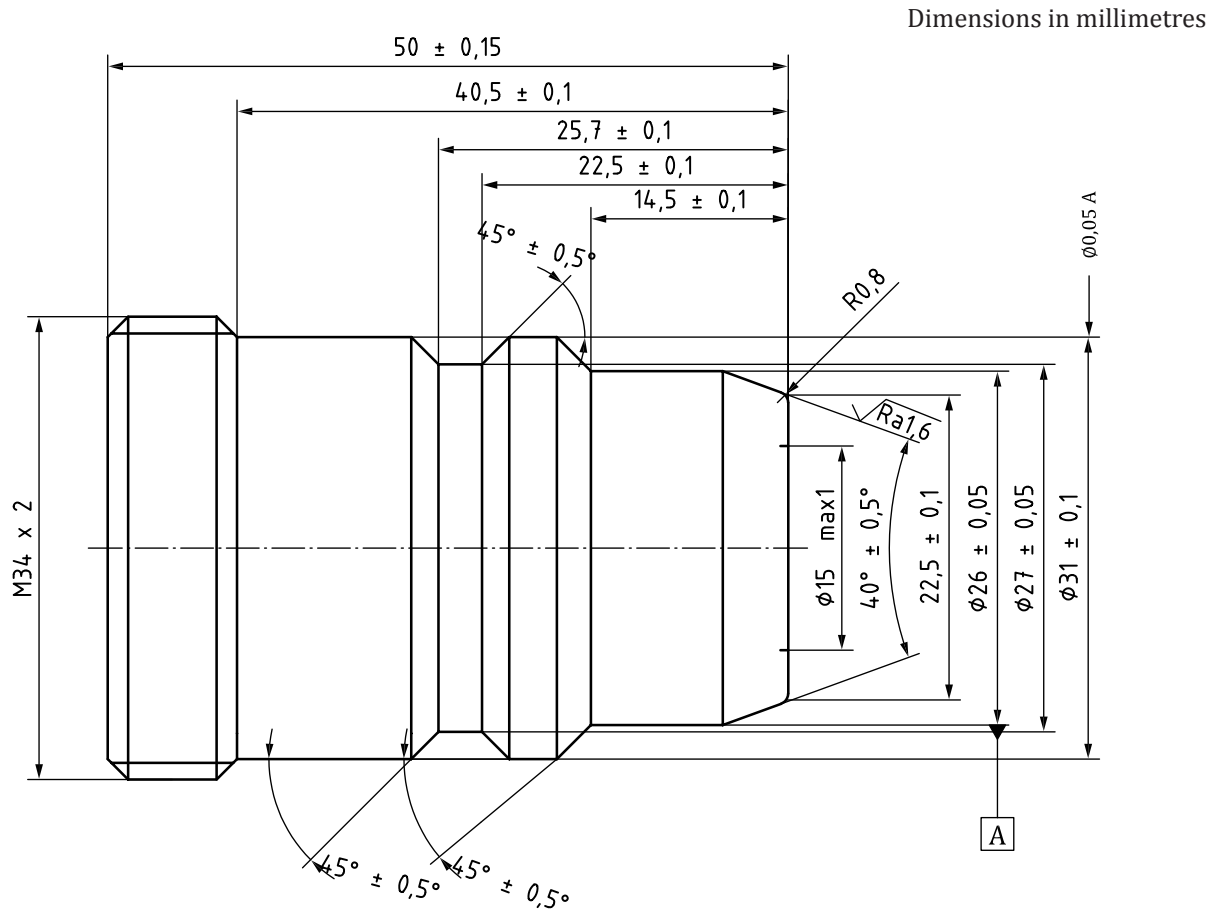
Figure 1 — D15 receptacle
