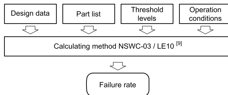
Figure 1 — Flow chart for calculating failure rates
