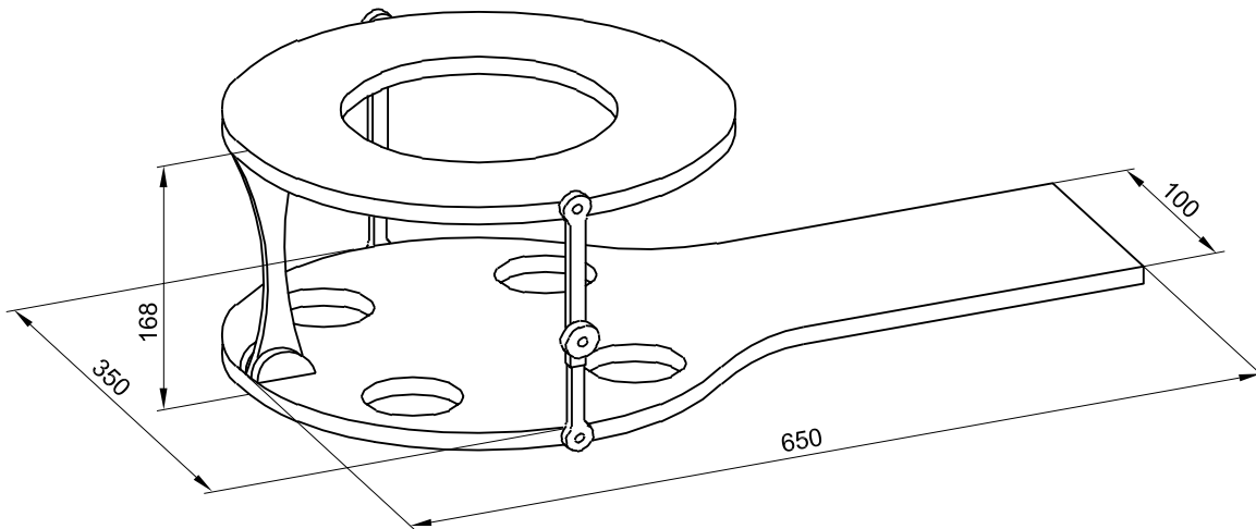
Figure 1 — Support apparatus
