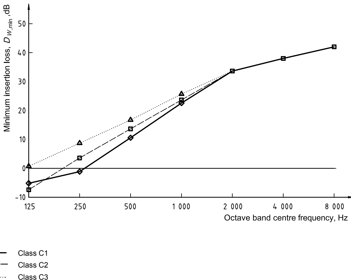
Figure 3 — Minimum insertion loss required for Class C
